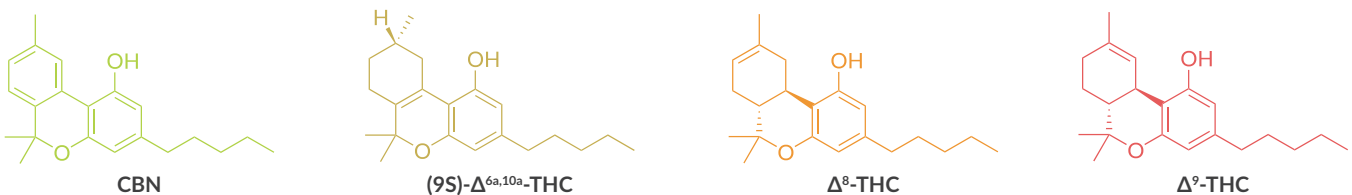
Figure 3. Atmospheric oxygen oxidizes \Delta^9 -THC to CBN and \Delta^8 -THC, as well as to other intermediates not shown above.
